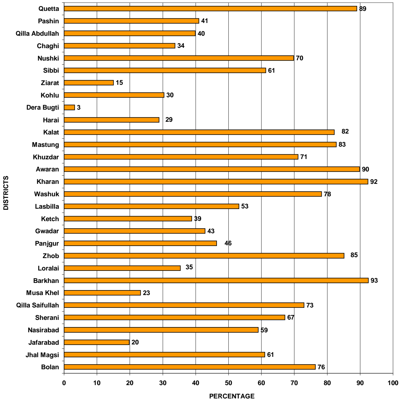
FIGURE 3.2 PERCENTAGE OF CHILDREN AGED 12-23 MONTHS THAT HAVE BEEN IMMUNISED C BASED ON RECALL AND RECORD FULLY IMMUNISED - BALOCHISTAN
